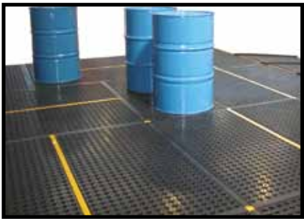
A BFFE2 & BFFE4 Workfloors connected using BFCO2 & BFCO3
